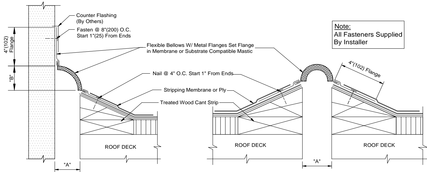
EJ-EEJ-100/100W THRU EJ-EEJ-2400/2400W DETAIL
