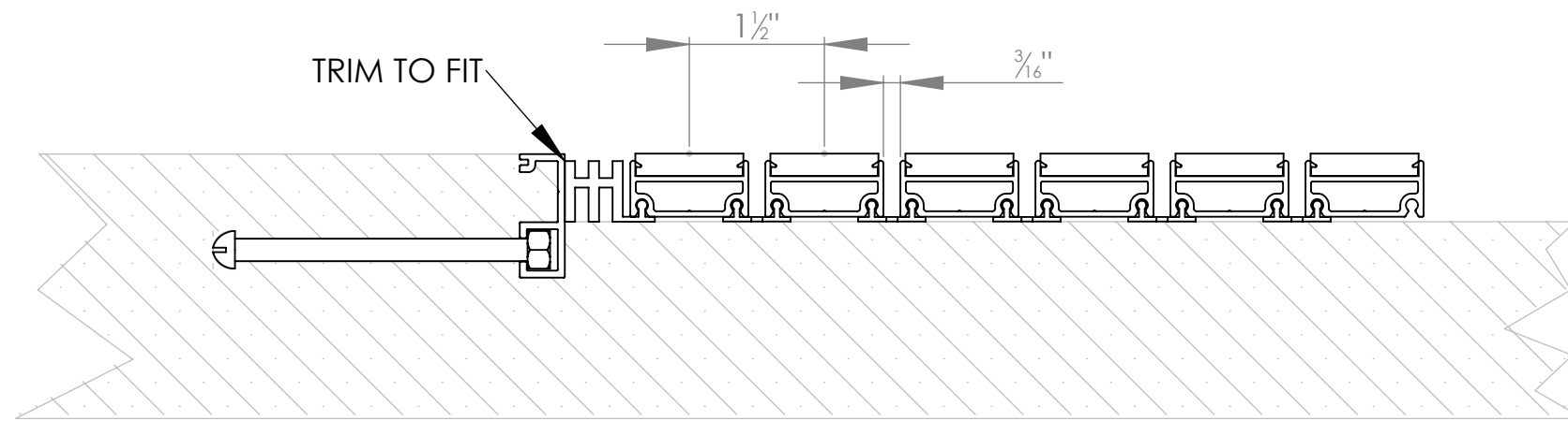
WIDTH VIEW
