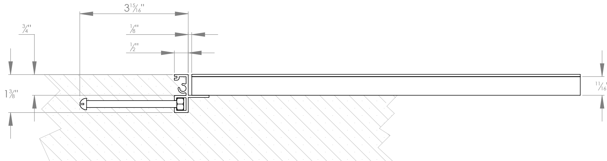
WIDTH VIEW
