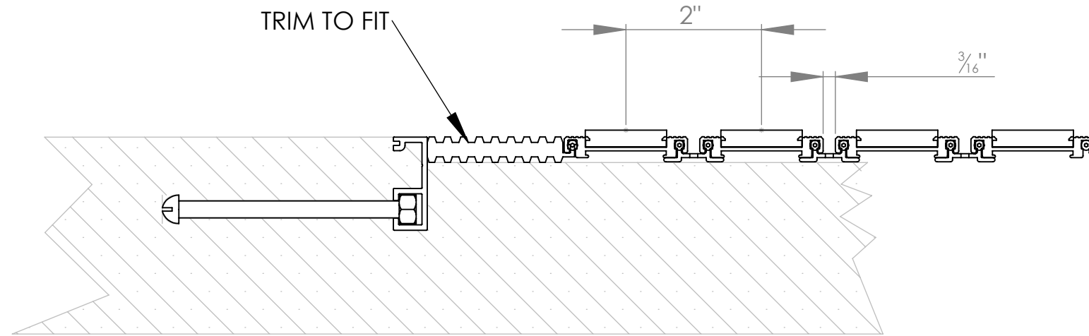
WIDTH VIEW
