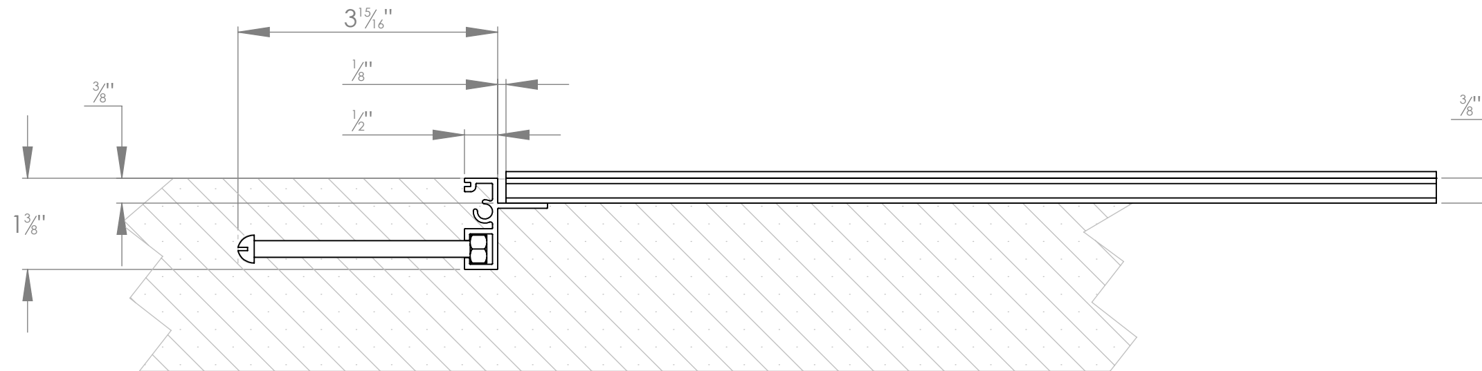
LENGTH VIEW
