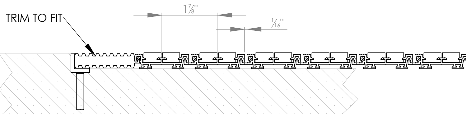
WIDTH VIEW
