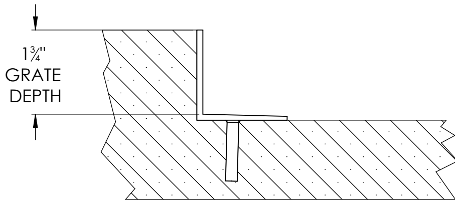
WIDTH VIEW
