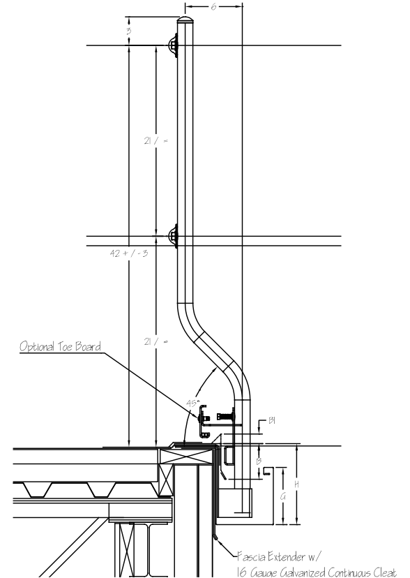
Gutter Edge on Exterior Wall
