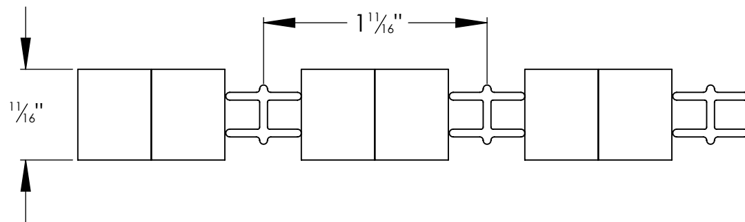
WIDTH VIEW
