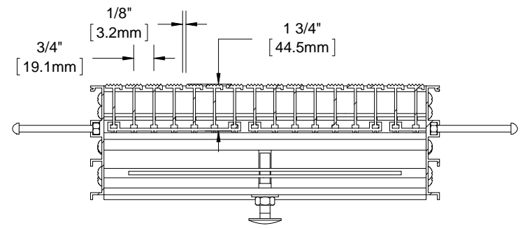
SECTION Y-Y
