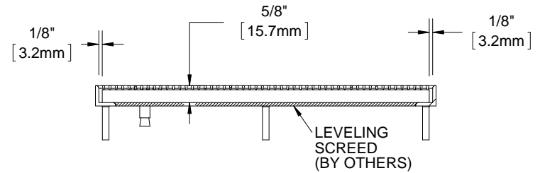
SECTION Y-Y
