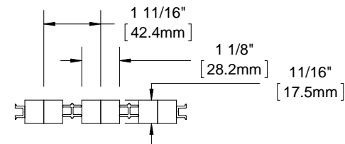
SECTION Y-Y SCALE 1 : 4
