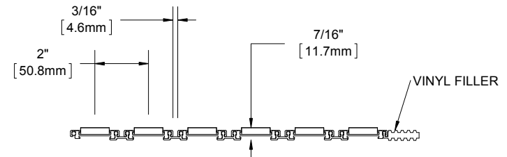
SECTION Y-Y
