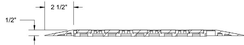
SECTION Y-Y
