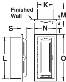
RECESSED
