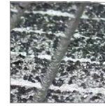
319 Cast Aluminum
