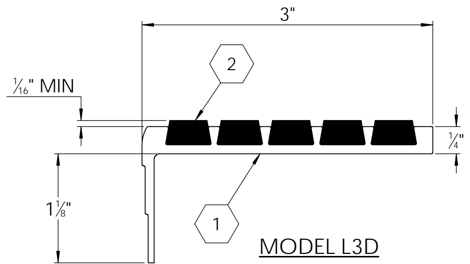
(SINGLE STAGE RIBBED ABRASIVE BARS)
