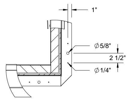
DETAIL G SCALE 1 : 15
