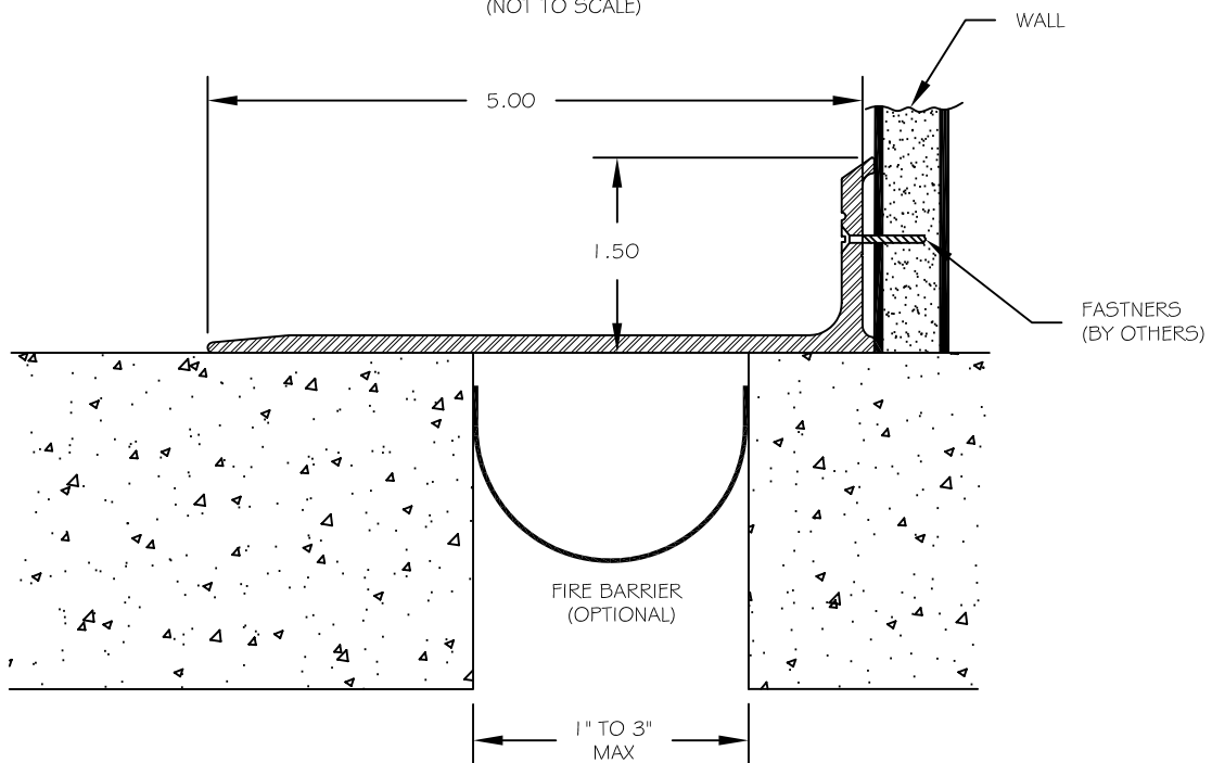
SURFACE CROSS SECTION (NOT TO SCALE)
