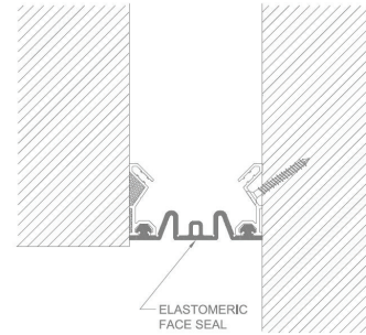
ELASTOMERIC FACE SEAL
