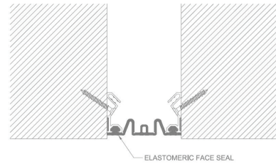
ELASTOMERIC FACE SEAL
