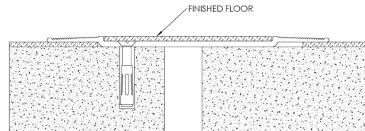
DOUBLE WING FLOORING INFILL SYSTEM
