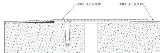
SINGLE WING FLOORING INFILL SYSTEM
