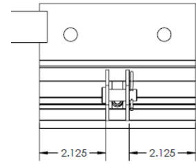
HINGE BRACKET CENTERED ON NUTRAIL
