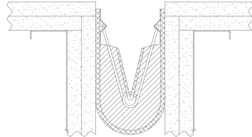
Inside Mount (standard) EJM-FLW140
