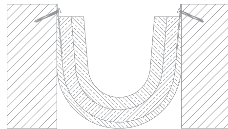
Inside Mount (standard) EJM-FLW
