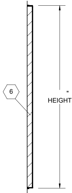
SECTION B-B
