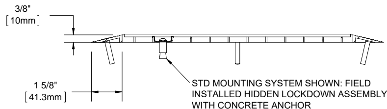
SECTION X-X
