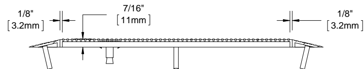
SECTION Y-Y
