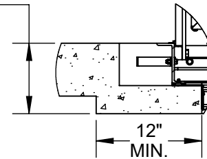
CAST-IN DETAIL
