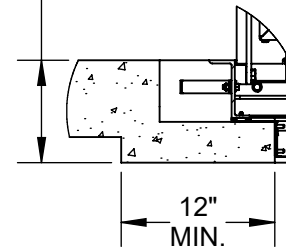
CAST-IN DETAIL
