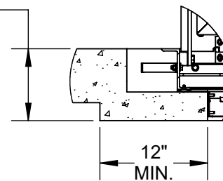
CAST-IN DETAIL
