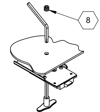
SLAM LATCH DETAIL
