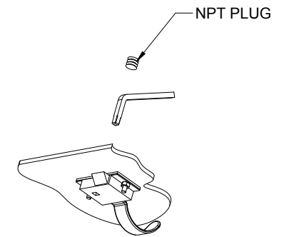
SLAM LATCH DETAIL
