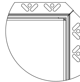
DETAIL D DRYWALL BEAD DETAIL SCALE 1 : 4
