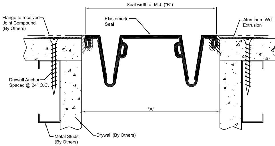
EJ-LCD-400/500/600 DETAIL WALL TO WALL CONDITION
