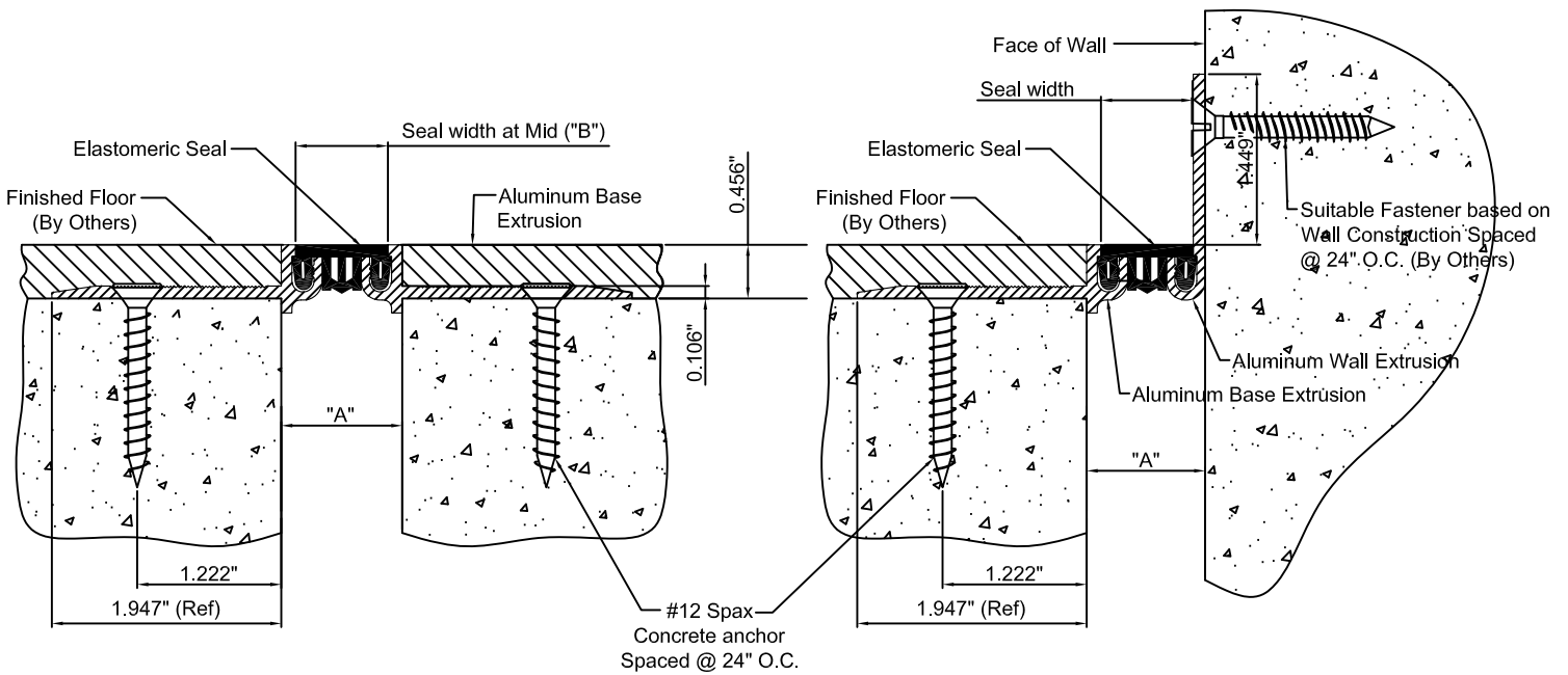
EJ-LCFC-100 DETAIL FLOOR TO FLOOR CONDITION
