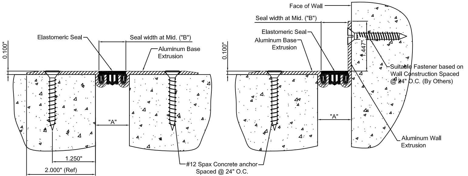
EJ-LCFS-100 DETAIL FLOOR TO FLOOR CONDITION
