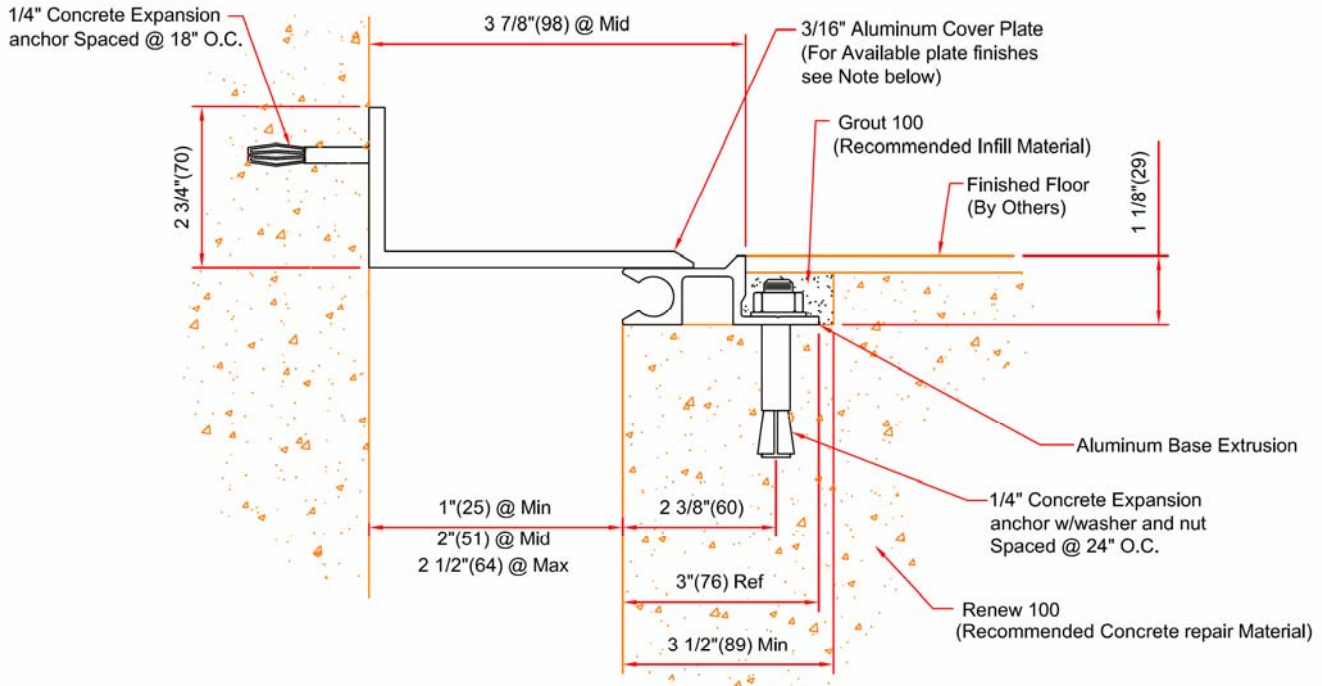
EJ-SFG-200W DETAIL FLOOR TO WALL CONDITION
