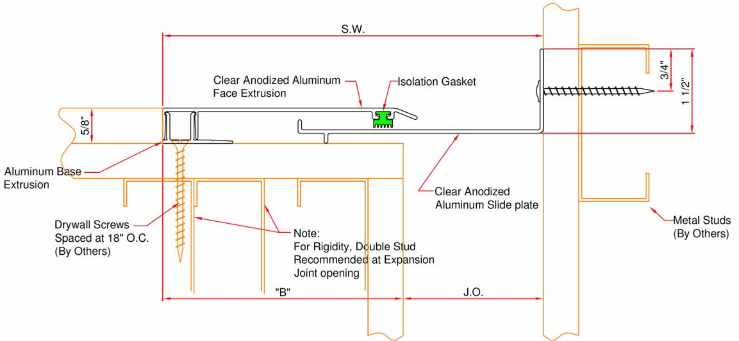
EJ-WCS-100W THRU EJ-WCS-300W WALL-TO-WALL CORNER CONDITION
