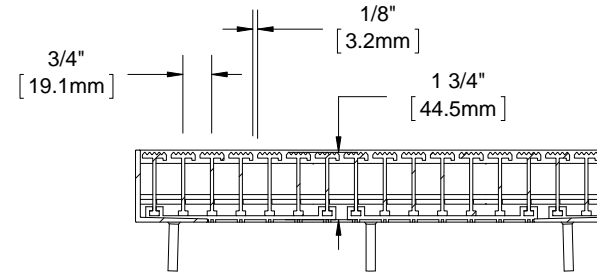
SECTION Y-Y
