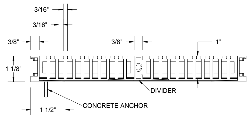
SECTION Y-Y
