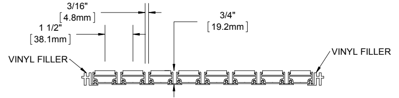
SECTION Y-Y
