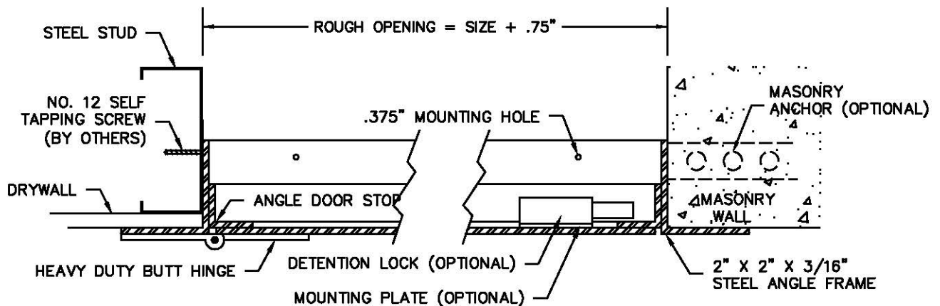
A A CUT-THRU SECTION NOT TO SCALE
