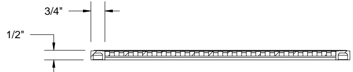
SECTION Y-Y
