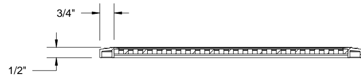
SECTION Y-Y
