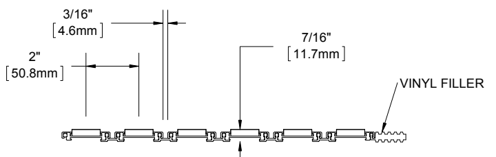
SECTION Y-Y
