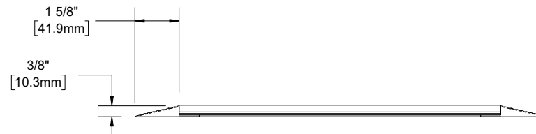
SECTION X-X
