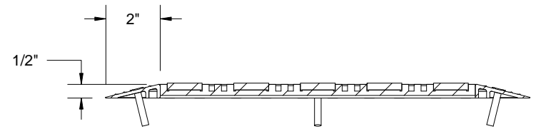
SECTION X-X
