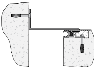
Floor-to-Wall/Corner Model: SFC/w
